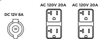
PLUG TYPES
